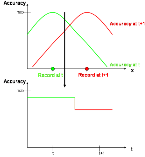
Figure 2: The location of the records has an impact on the spatial accuracy of the lighting reconstructed by irradiance caching compared to a reference solution. Since irradiance caching is based on sparse sampling and extrapolation of incoming radiance, the accuracy of the solution at a given point (marked by the black arrow) is not constant over a surface. When records are located at different points in successive frames, the accuracy at a given point can change abruptly. Therefore, the incoming radiance can change noticeably between two frames, yielding flickering artifacts. The maximum accuracy is obtained at the point and time of actual computation of the incoming radiance.
